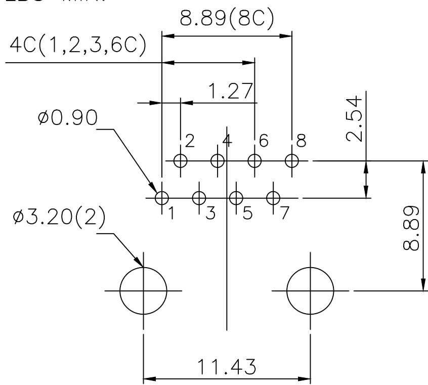
OPTION OF 10P8C AND 10P4C PC Board Layout t = 1.60mm Component Side Shown Tolerance ±0.05mm
