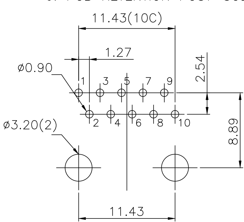
OPTION OF 10P10C PC Board Layout t = 1.60mm Component Side Shown Tolerance ±0.05mm
